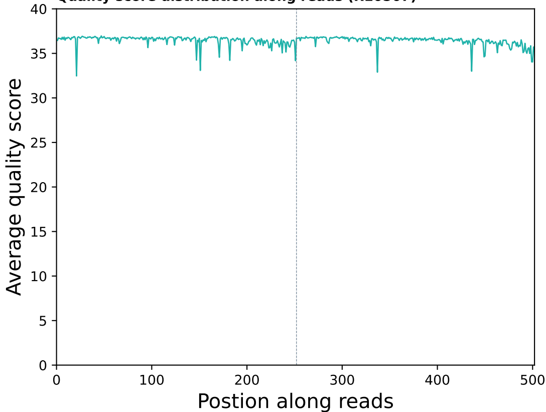
Quality score distribution along reads (R10507)
